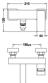
方形浴用龍頭 8.24.022 $6,700
